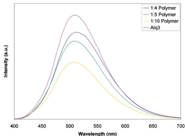
Figure 1. Emission spectra in \text{CHCl}_3 excited at 380 nm.
